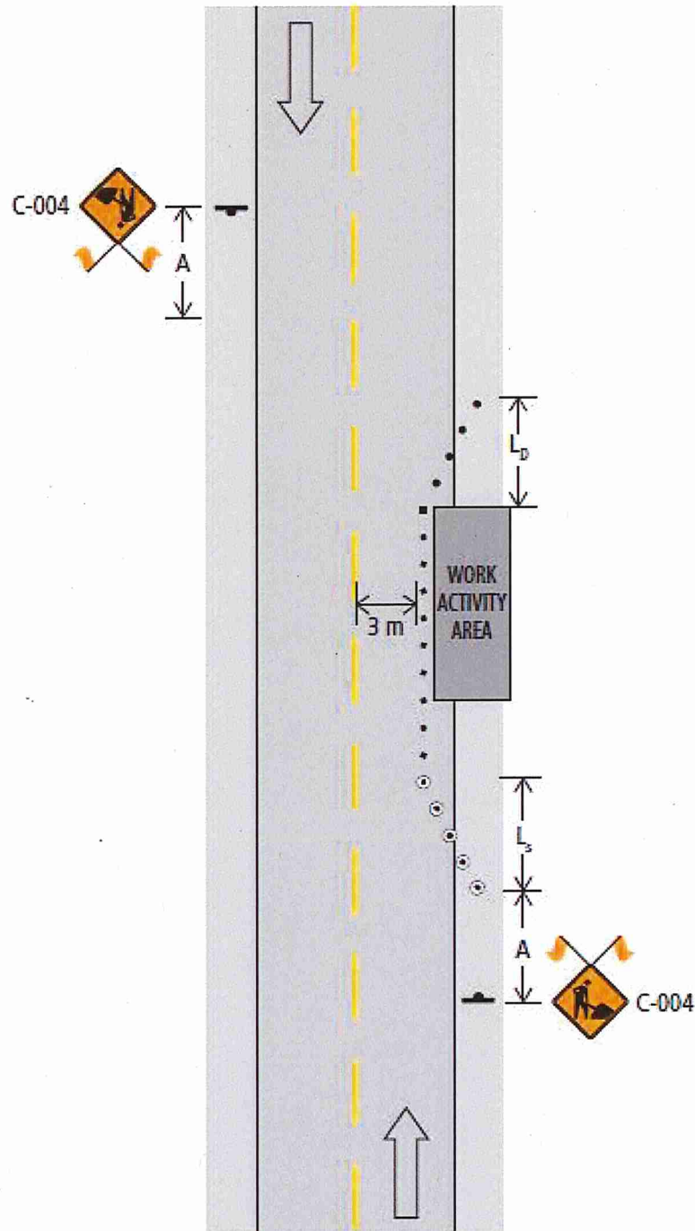
Figure 7.7: Roadside Work – Encroachment into Travel Lane – Short Duration
